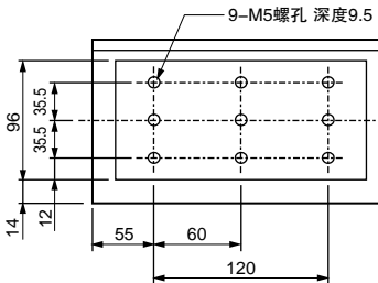
①SGLFW-1Z□200B□□
