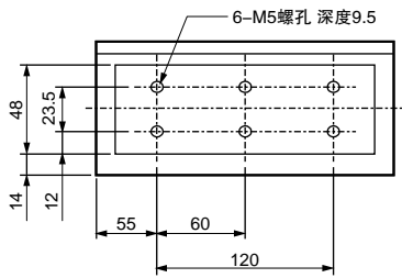
① SGLFW-50□200B□
