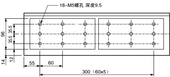
②SGLFW-1ZD380B□□
