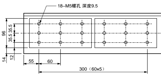
② SGLFW-1Z□380B□
